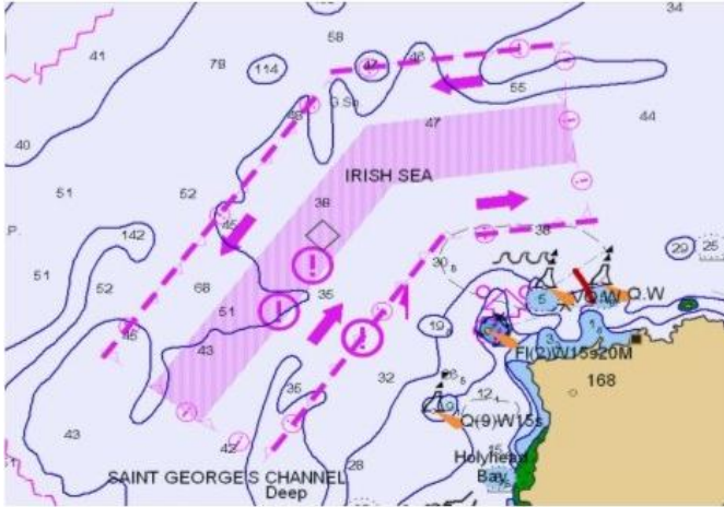
Figure 25 – Traffic Separation Scheme with appropriate masking
