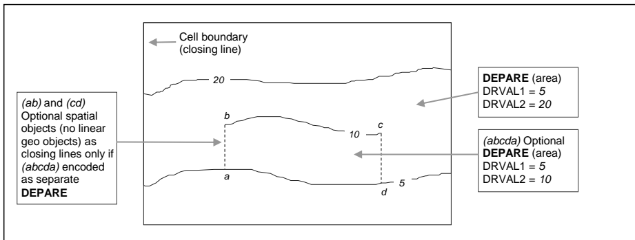
Figure 5 – Geometry of depth areas
