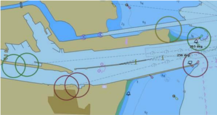
Figure 16 – Omnidirectional light display in ECDIS
