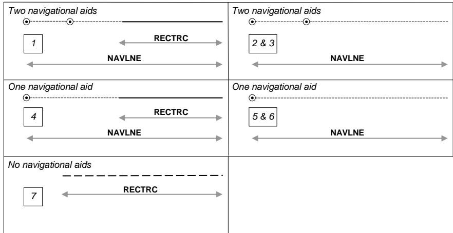
Figure 10 – Navigation lines and recommended tracks
