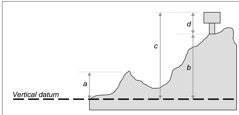
Figure 1 – Heights and elevations
