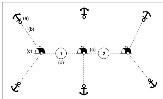
Figure 9 – Mooring trot
