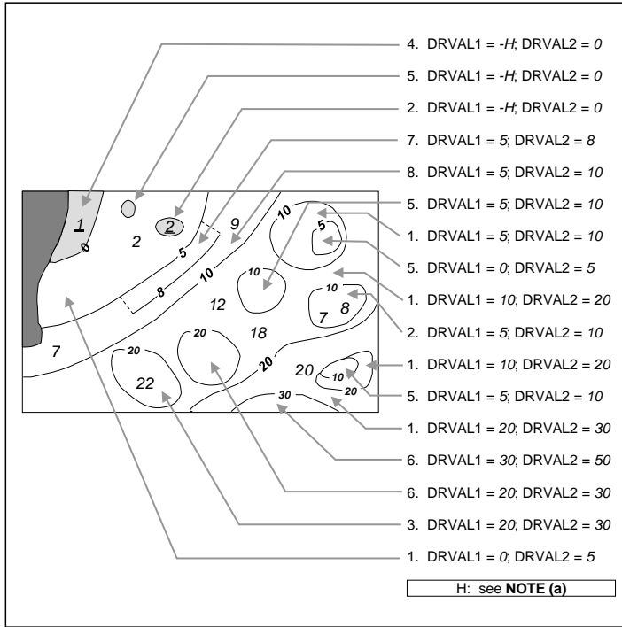
Figure 6 – Depth areas
