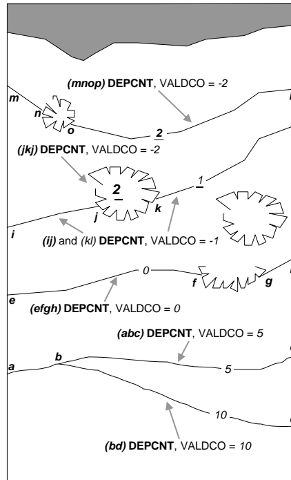
Figure 4 – Depth contours
