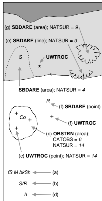
Figure 8 – Seabed areas
