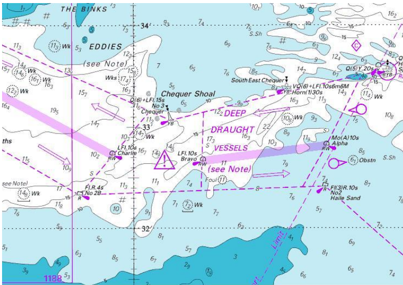
Example of a raster chart
