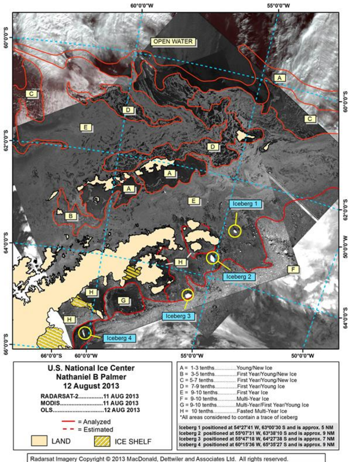
Figure 13.3: Example of a multi-source satellite annotated Imagery for the Antarctic peninsula area
