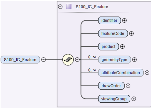
Figure 11-6. Structure of S100_IC_Feature
