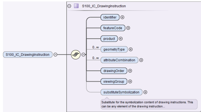
Figure 11-7. Structure of S100_IC_DrawingInstruction
