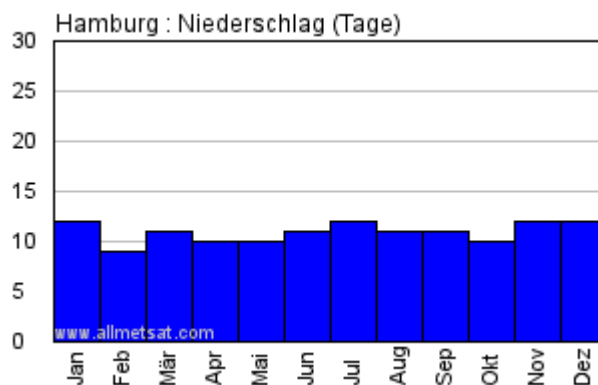
Figure 2: Days with precipitation ≥ 1 mm
