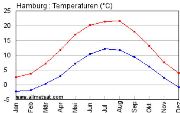
Figure 1: Average daily minimum and maximum temperature.
