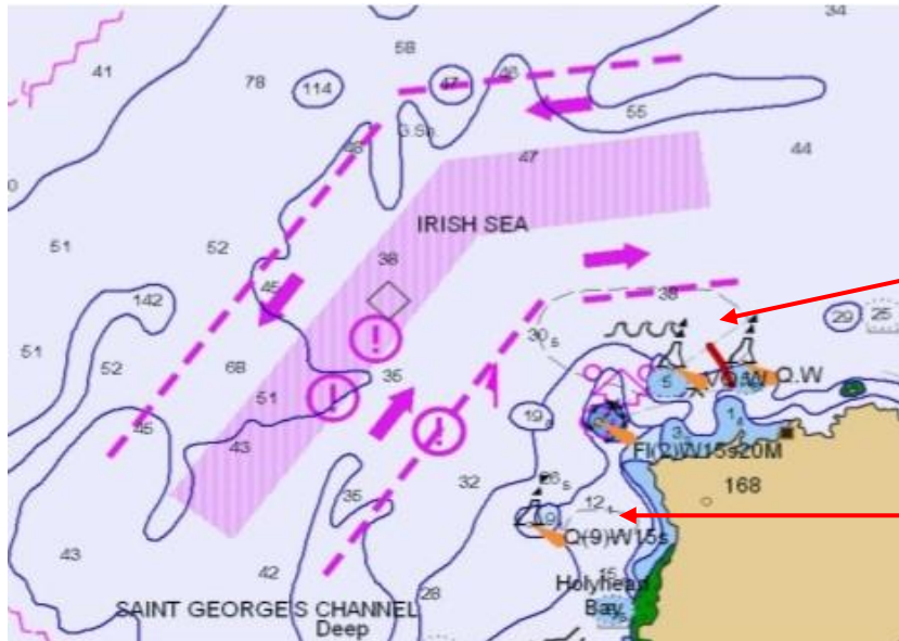
Traffic Separation Scheme with masked Caution Area
