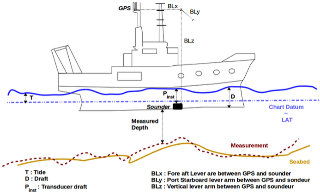
Figure 5. Effects of not correcting for horizontal offsets. Here, not measuring the horizontal offset between the GNSS receiver position and the echo sounder results in along-track offsets of seafloor features. Red line: measured; yellow line: reality.
