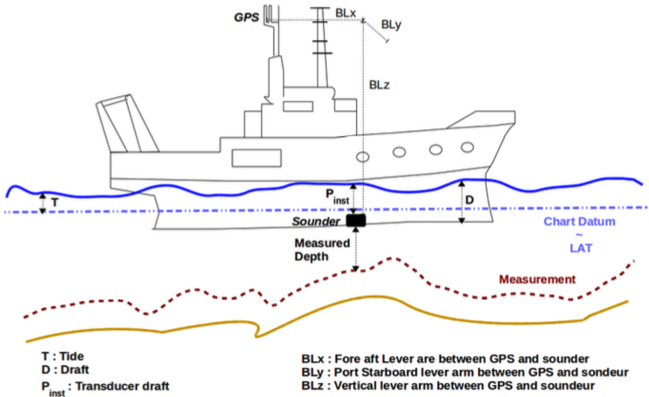
Figure 4. Examples of the effects of not correcting for vertical offsets. Here, not correcting for the offset of the transducer from the waterline leads to a measurement (red line) that differs significantly from reality (yellow line). This gives a bias (systematic) uncertainty to the measurements.
