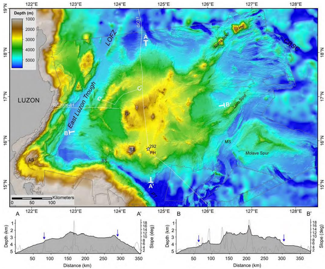
Fig 2: Morphostructural characteristics of the Apolaki caldera in red . BB = Benham Bank:
