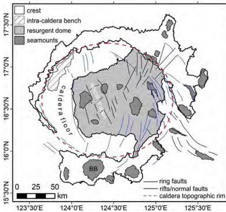
Fig 2: Morphostructural characteristics of the Apolaki caldera in red . BB = Benham Bank:
