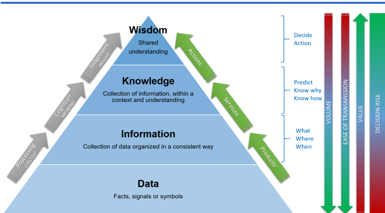
Figure 1: Data-Information-Knowledge-Wisdom Pyramid
