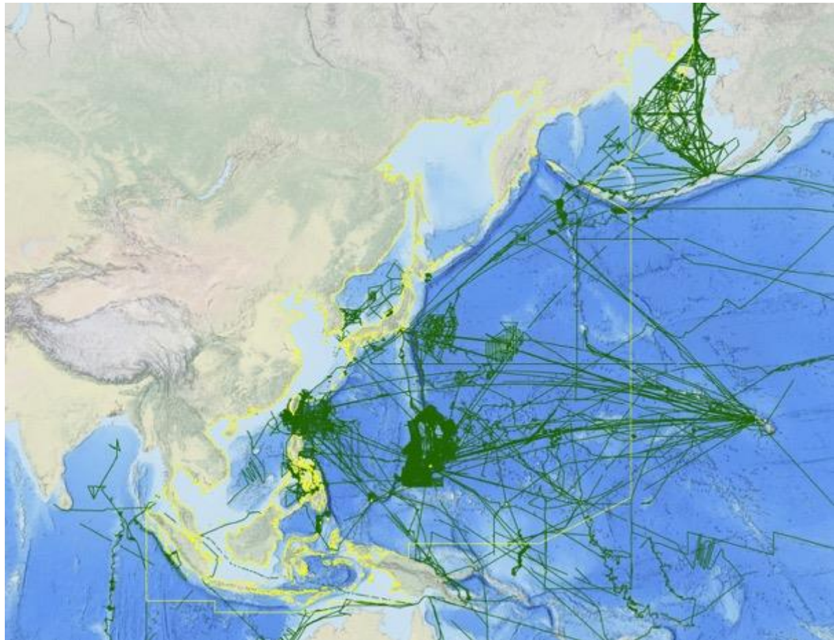
Figure 1: Multibeam bathymetric ship tracks (green lines) of IHO DCDB data holdings in the EAHC Region commensurate with IHO INT Region K (yellow polygon).
