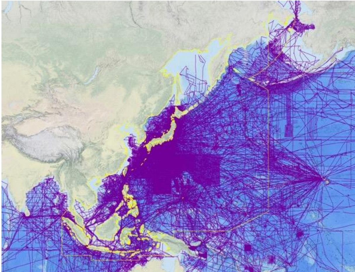
Figure 2: Singlebeam bathymetric ship tracks (purple lines) of IHO DCDB data holdings in the EAHC Region commensurate with IHO INT Region K (yellow polygon).
