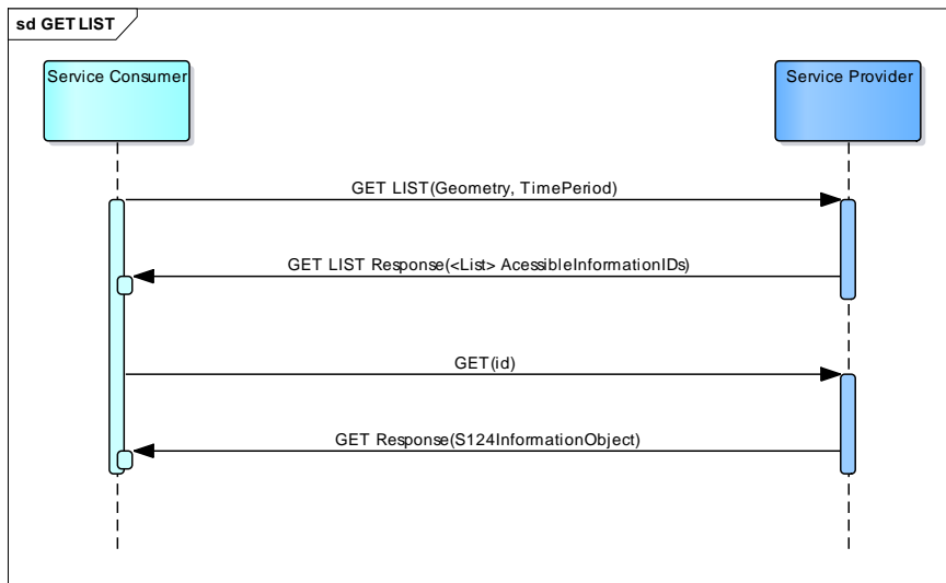
Figure 2 Manual retrieval of Navigational Warnings (needs update).
