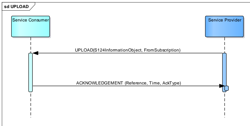
Figure 3 Upload message initiated by service provider with acknowledgement.
