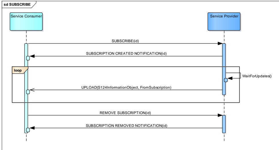
Figure 4 Subscription requested by external service
