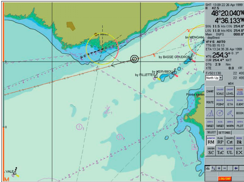
Base Display, day
