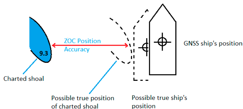
Figure 4-2 – Horizontal position accuracy accounting for ZOCs and ship's GNSS position
