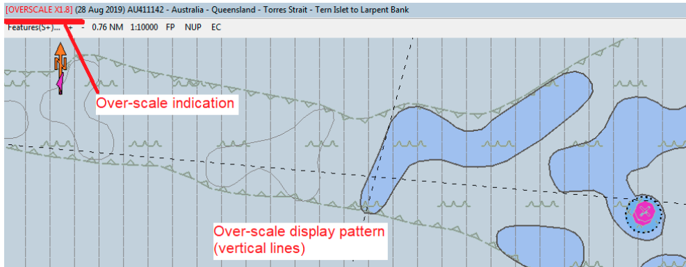
Figure 7: Over-scale indication and over-scale pattern on ECDIS
