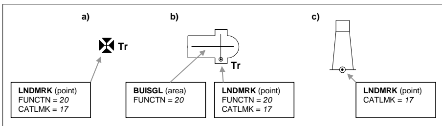
Figure 3 - Landmarks
