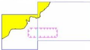
Figure 20 – Area object crossing ENC cell boundaries
