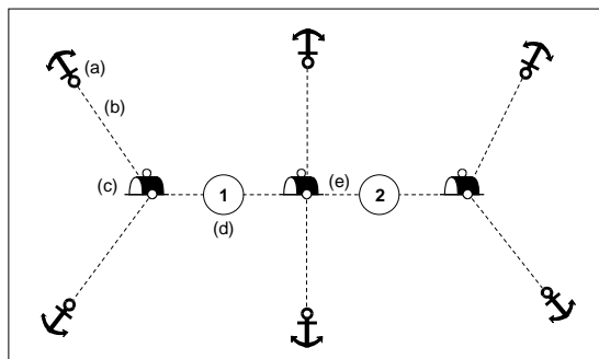
Figure 9 – Mooring trot
