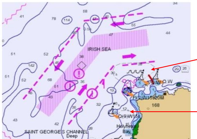
Figure 26– Traffic Separation Scheme with masked CTNARE
