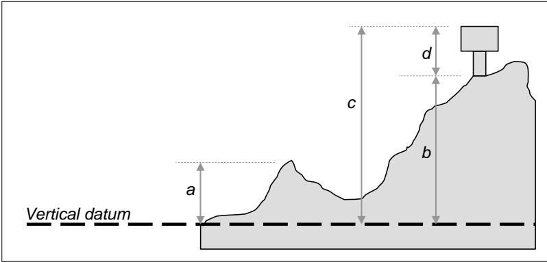
Figure 1 – Heights and elevations
