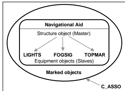
Figure 15 – Navigational aids
