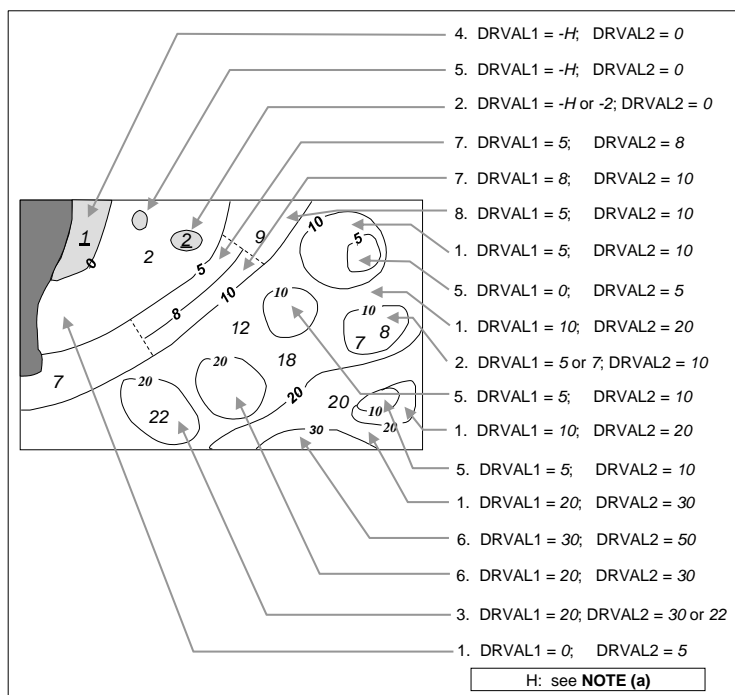
Figure 6 – Depth areas
