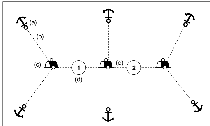
Figure 9 – Mooring trot
