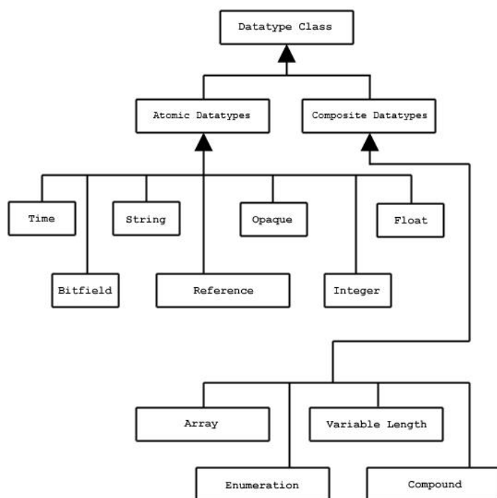
Figure 10c-5 - Datatype classifications
