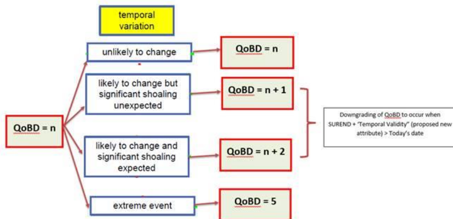
Proposed logic for ECDIS downgrading of charted QoBD features.
