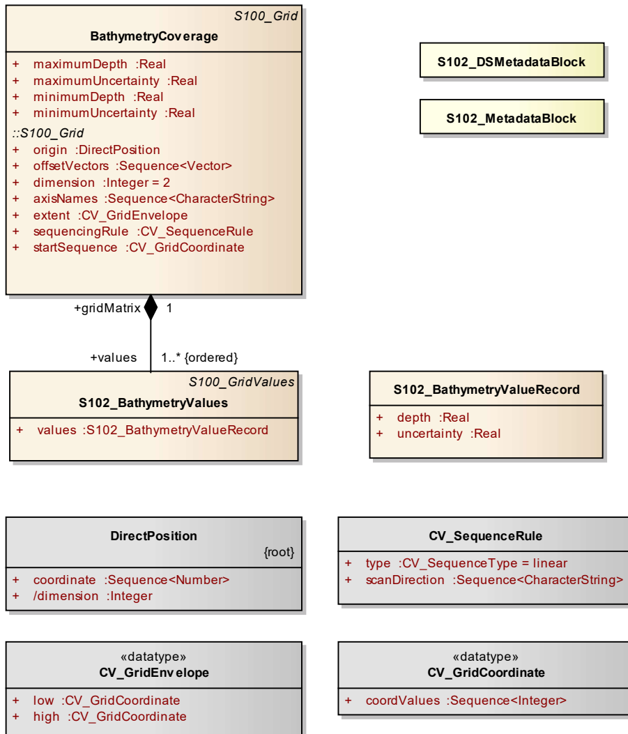
Figure 4-4 - Implementation of Classes of S-102
