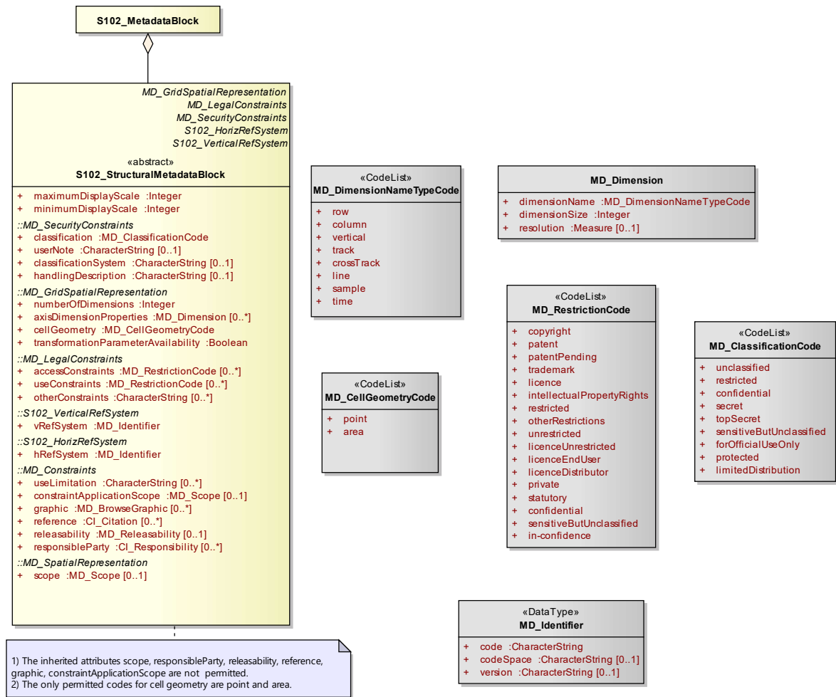
Figure 12-2 - S-102 Structure Metadata
