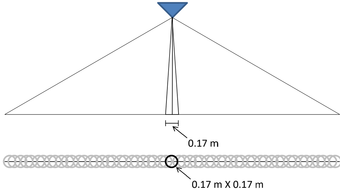
Figure H 1 – Sonar Footprint at Nadir
