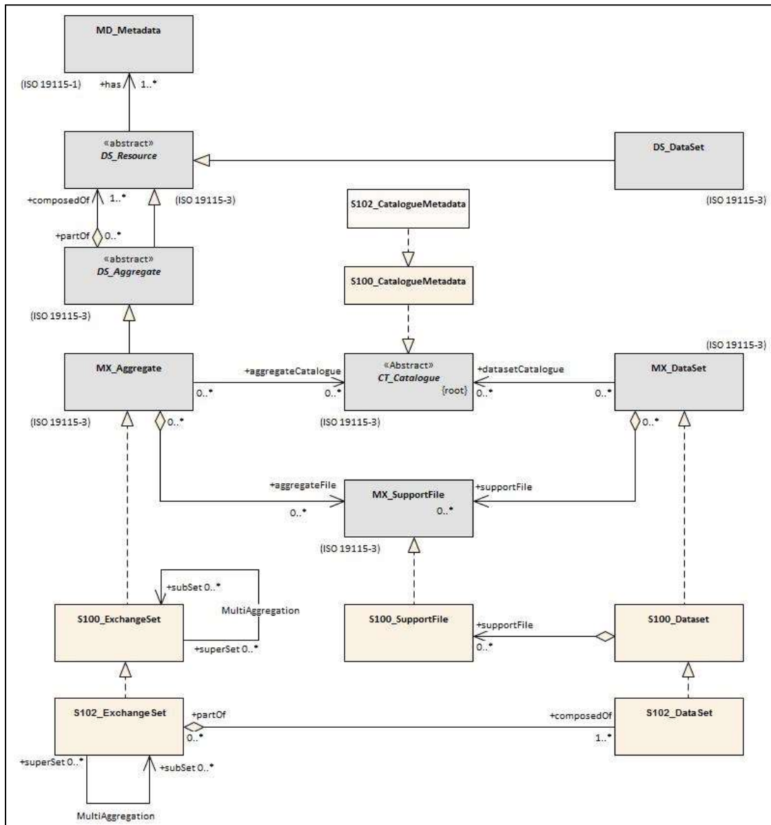
Figure 12-4 - Realization of the Exchange Set classes
