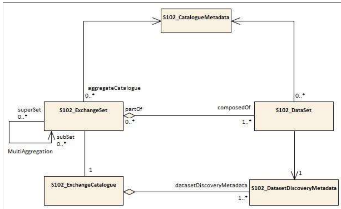
Figure 12-6 - S-102 Exchange Set
