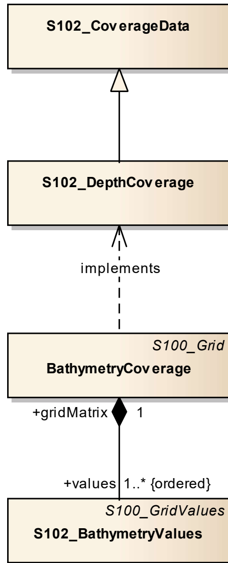
Figure 4-3 - Coverage Structure of S-102
