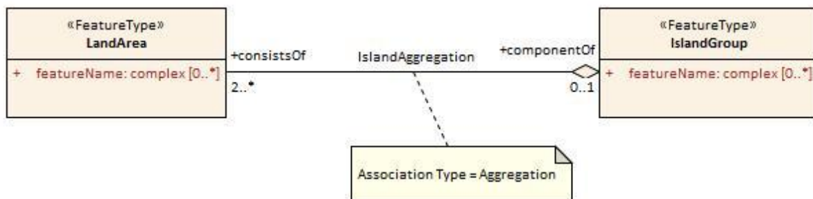
Figure 4-2 – Aggregation
