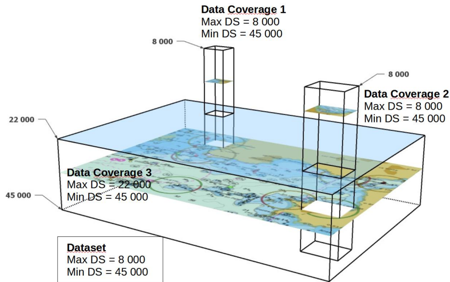
Figure 4-6 – Dataset with multiple Data Coverage features
