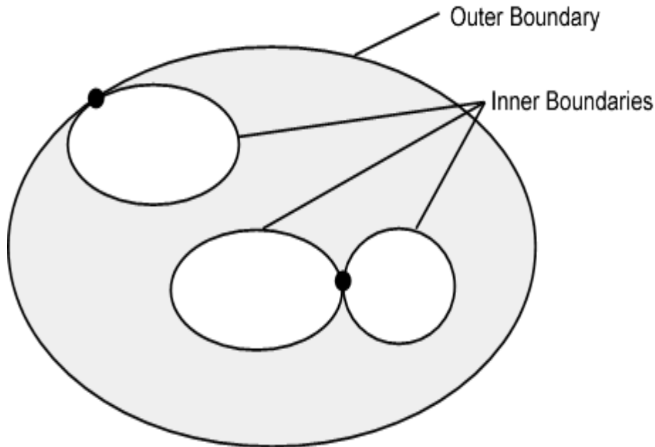
Figure 4-12 – Area Holes
