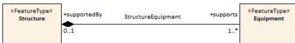
Figure 4-3 – Composition
