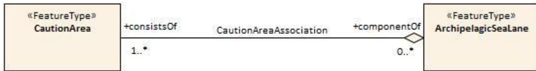
Figure 4-1 – Feature association
