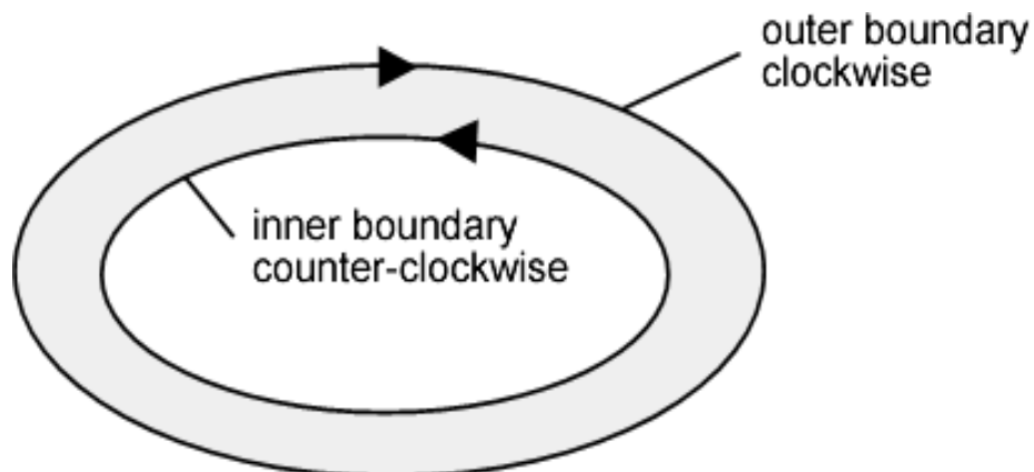
Figure 4-13 – Boundary direction
