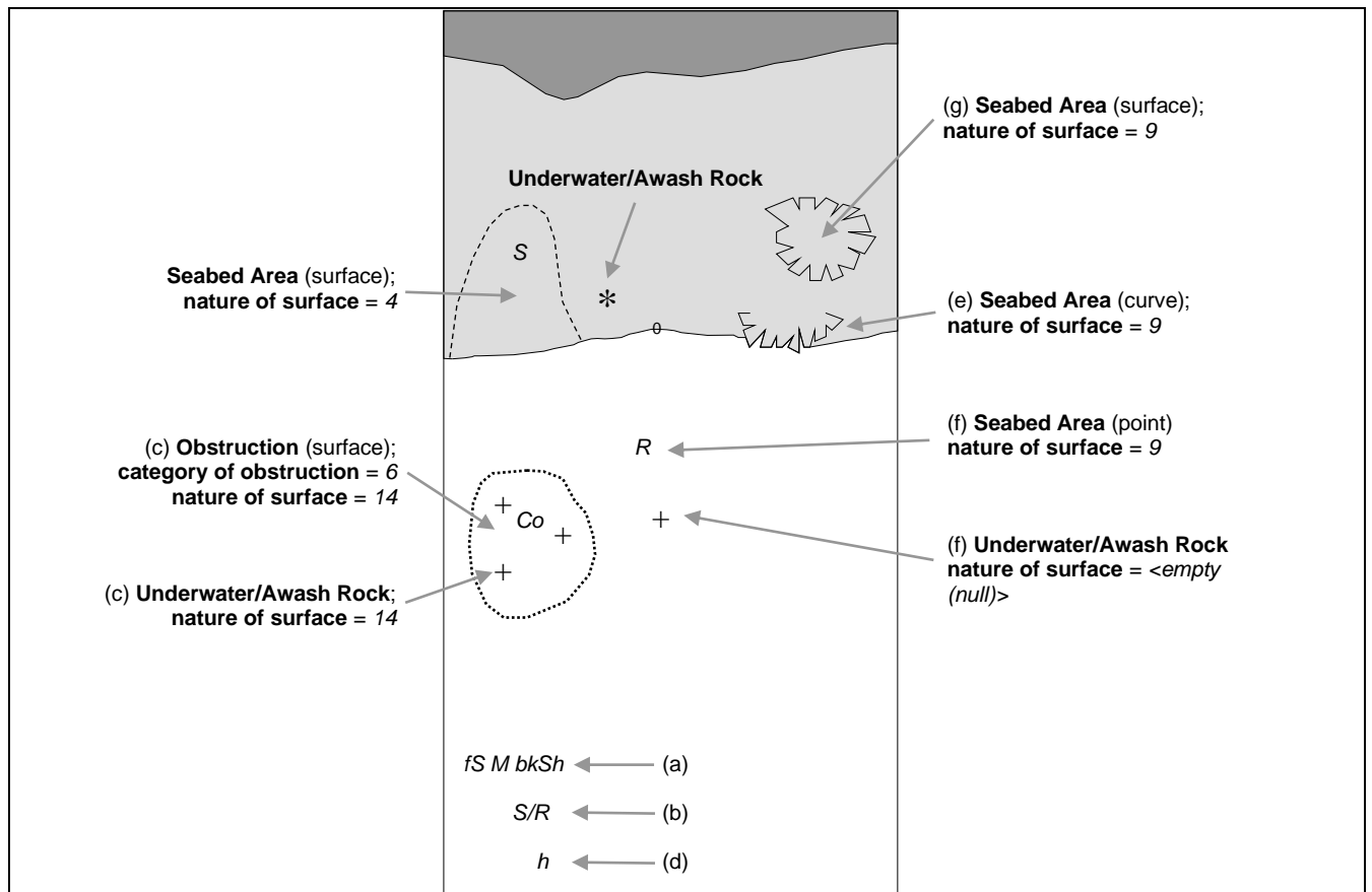
Figure 12-1 – Seabed areas
