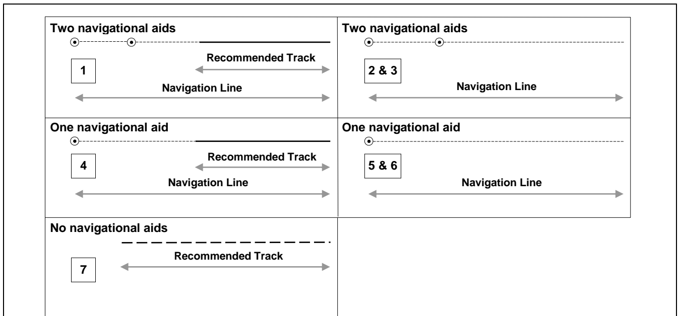
Figure 15-4 – Navigation lines – Geometry encoding
