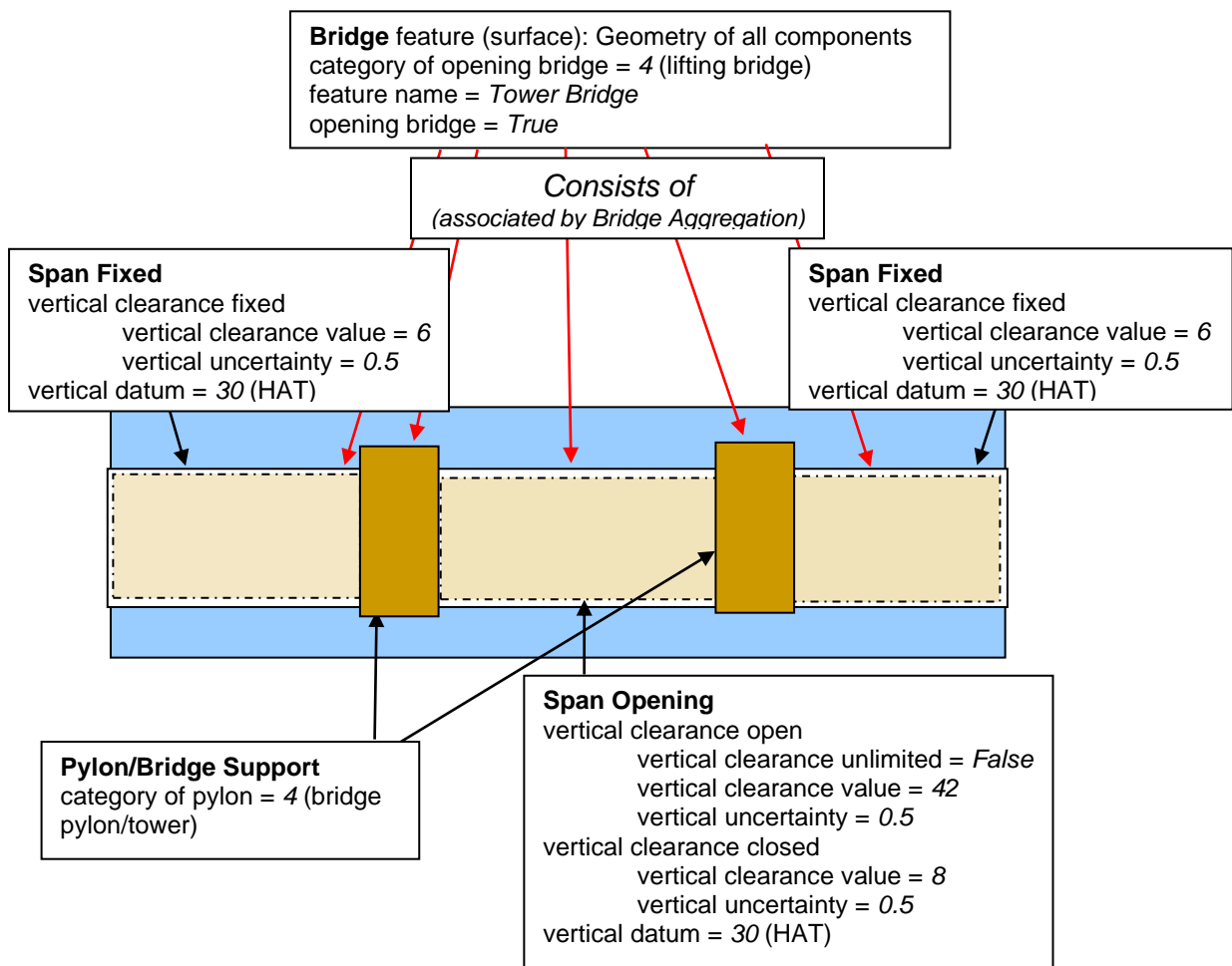
Figure 6-2 - Lifting bridge – Example
