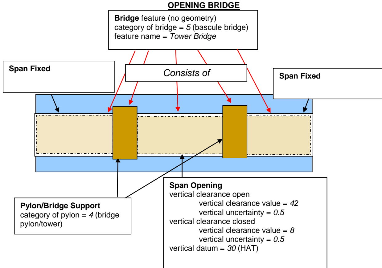
Figure 6.2 - Opening bridge - Example
