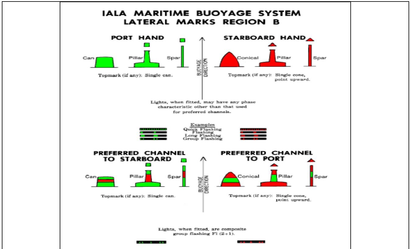
Figure 20.1 - IALA lateral buoys - Characteristics
