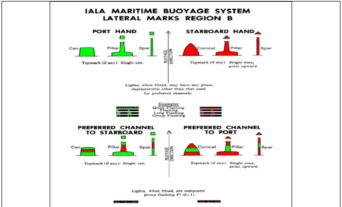
Figure 20.5 - IALA lateral beacons - Characteristics
