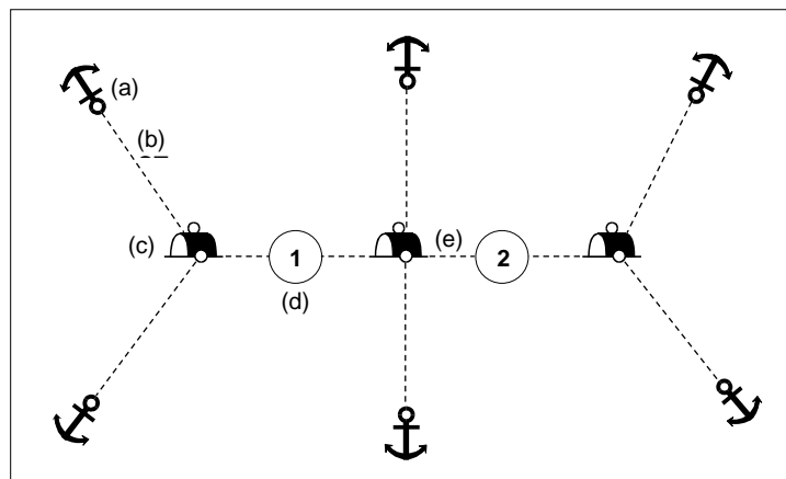
Figure 8.2 - Mooring trot
