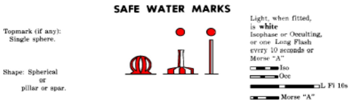
Figure 20.4 - IALA safe water buoys - Characteristics
