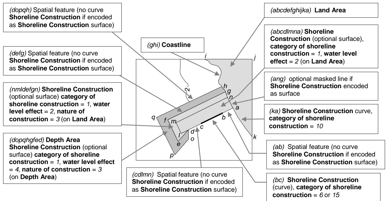
Figure 8.1 - Shoreline constructions
