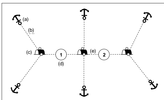
Figure 8.2 - Mooring trot
