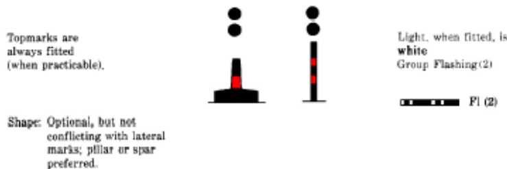
Figure 20.7 - IALA isolated danger beacons - Characteristics
