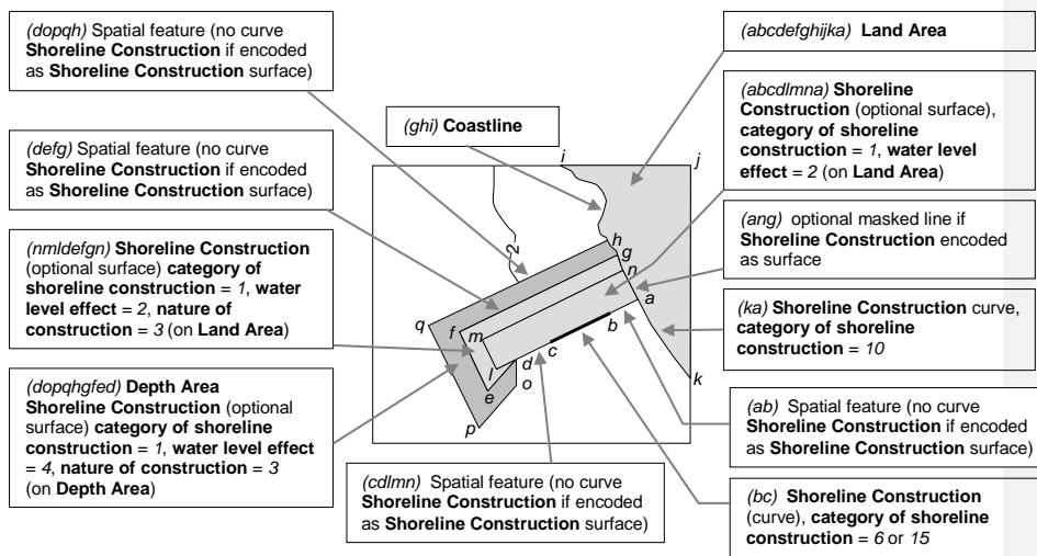
Figure 8.1 - Shoreline constructions
