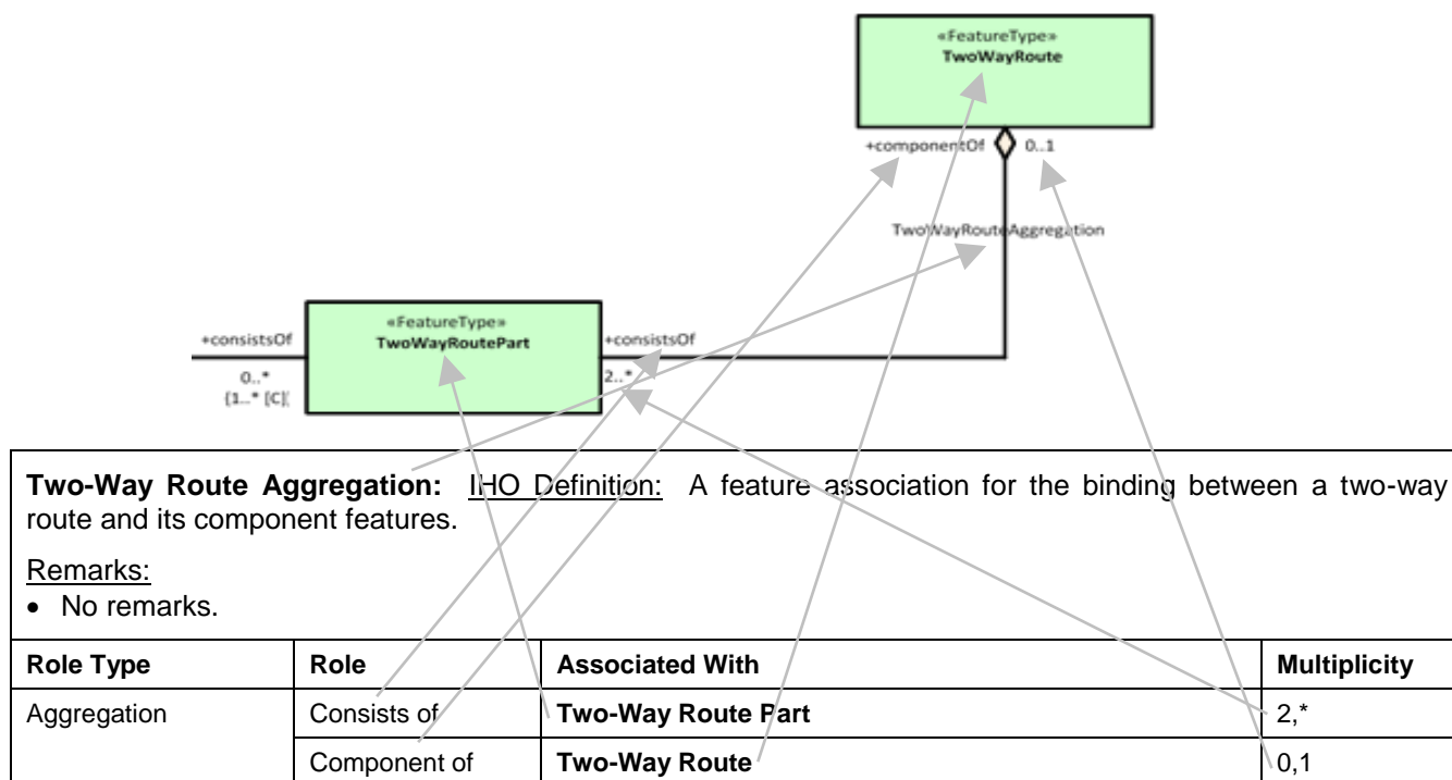
Figure 25.2 – Two-Way Route Aggregation
