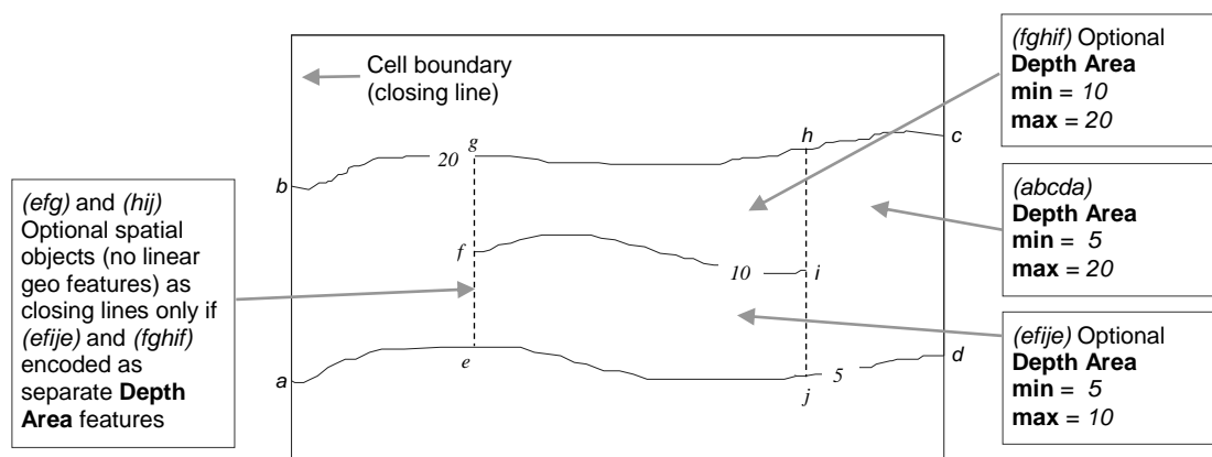
Figure 11.3 - Geometry of depth areas
