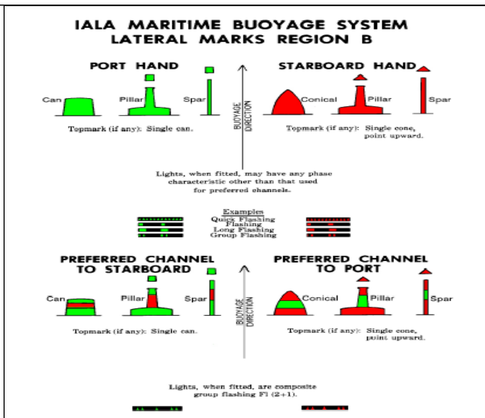
Figure 20.5 - IALA lateral beacons - Characteristics
