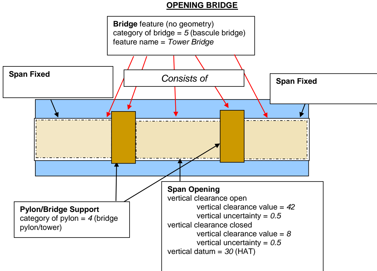
Figure 6.2 - Opening bridge - Example
