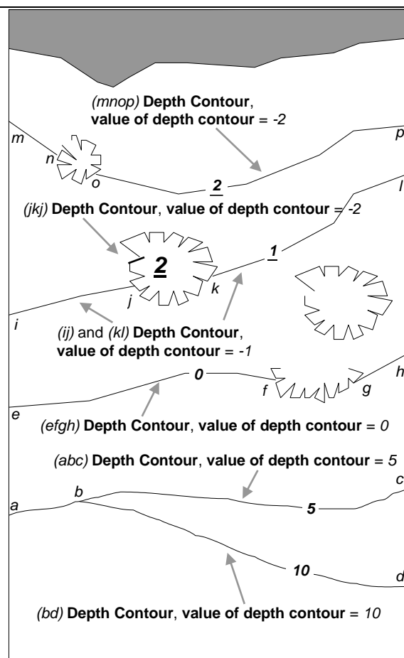
Figure 11.2 - Depth contours
