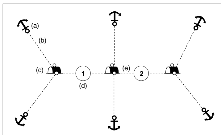
Figure 8.2 - Mooring trot
