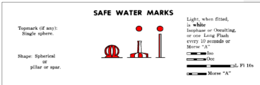
Figure 20.4 – IALA safe water buoys – Characteristics
