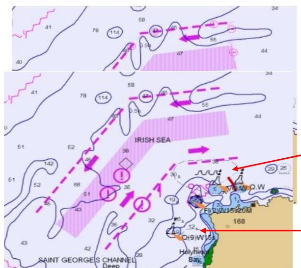
Figure 2.10 - Traffic Separation Scheme with appropriate masking
