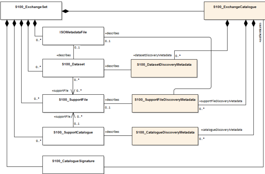
Figure 11-1 – Exchange Set Structure
