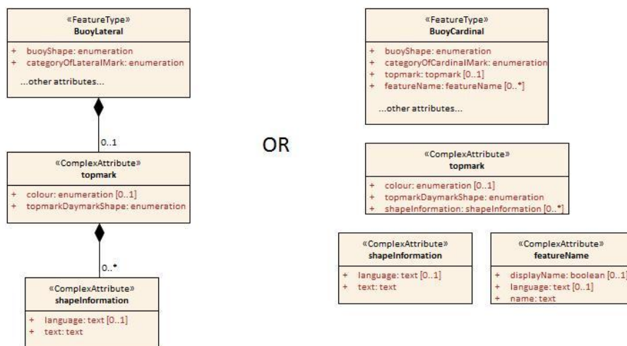
Figure 4-6 – Complex attribute
