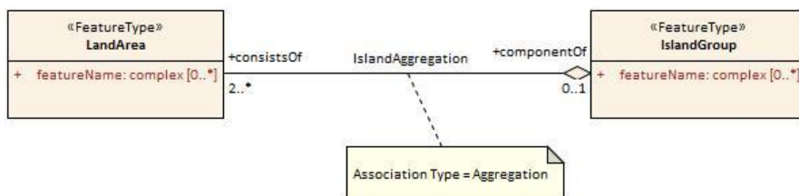
Figure 4-2 – Aggregation
