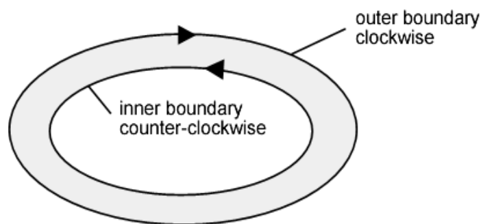
Figure 4-15 – Boundary direction
