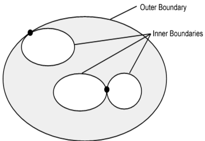
Figure 4-14 – Area Holes
