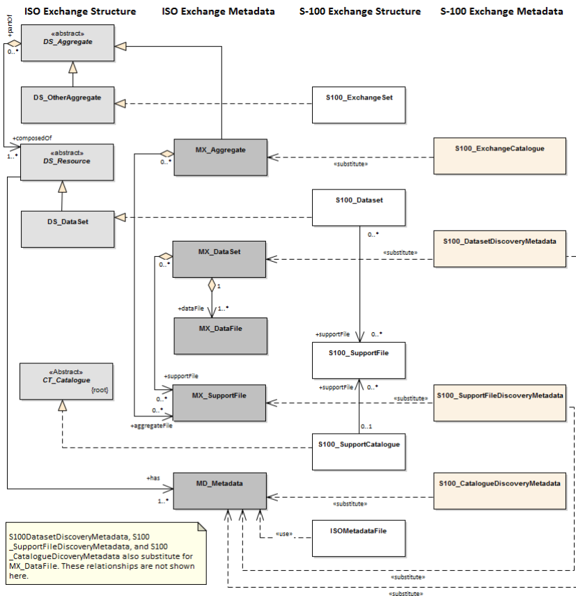
Figure 12-1 – Realization of the Exchange Set classes
