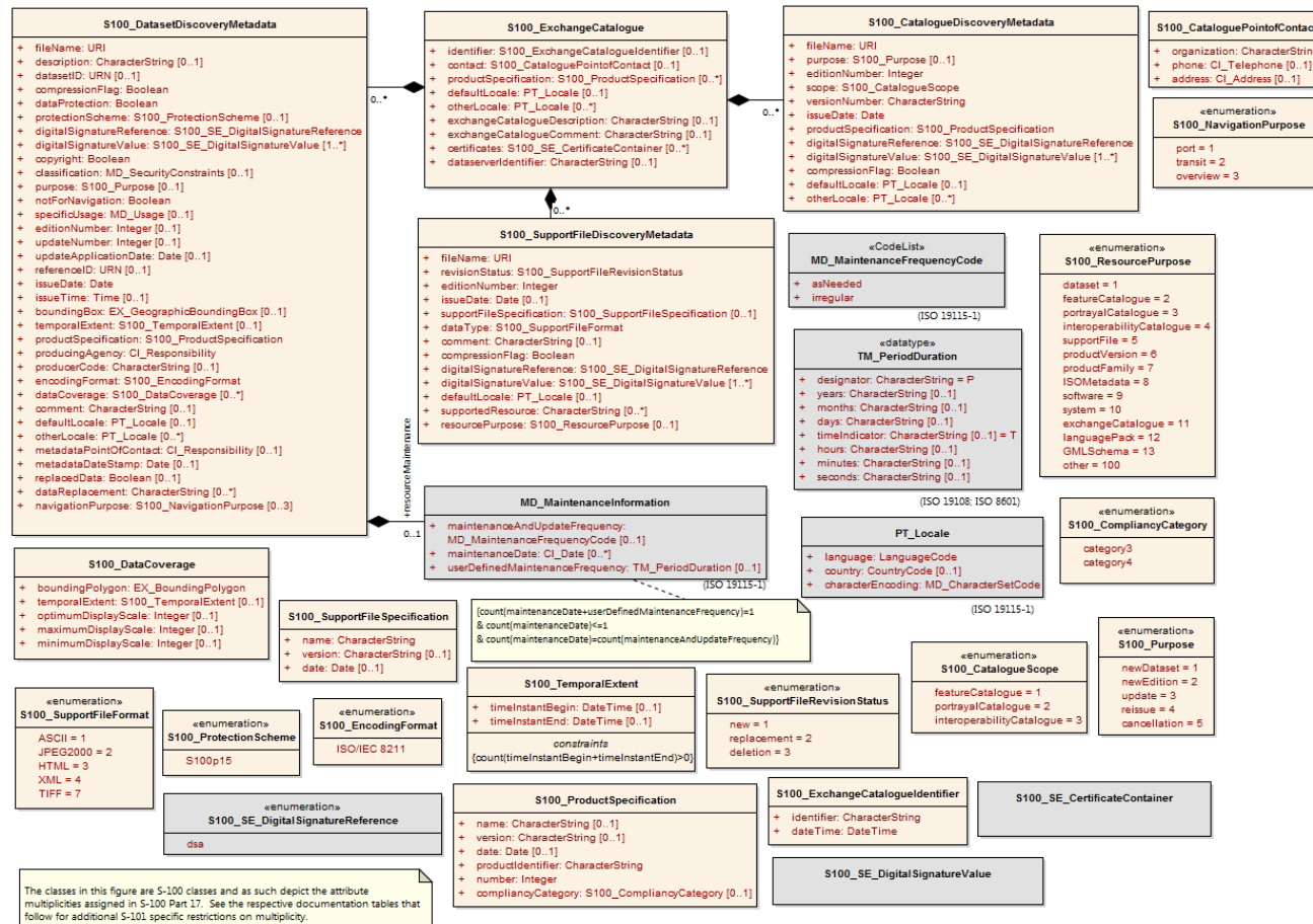
Figure 12-3 – S-101 Exchange Set - class details
