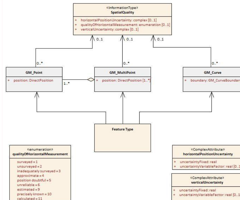
Figure 4-5 – Spatial Quality information type
