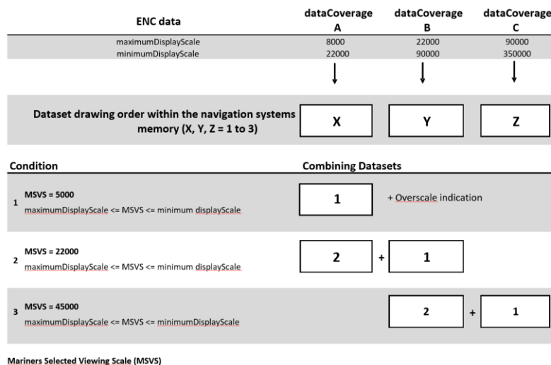
Figure 4-9 – Dataset loading and display rules
