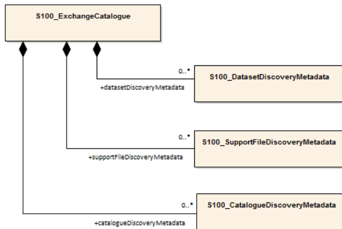
Figure 12-2 – S-101 Exchange Set Catalogue
