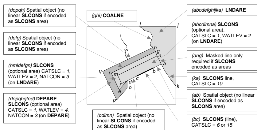
Figure 2 – Shoreline constructions
