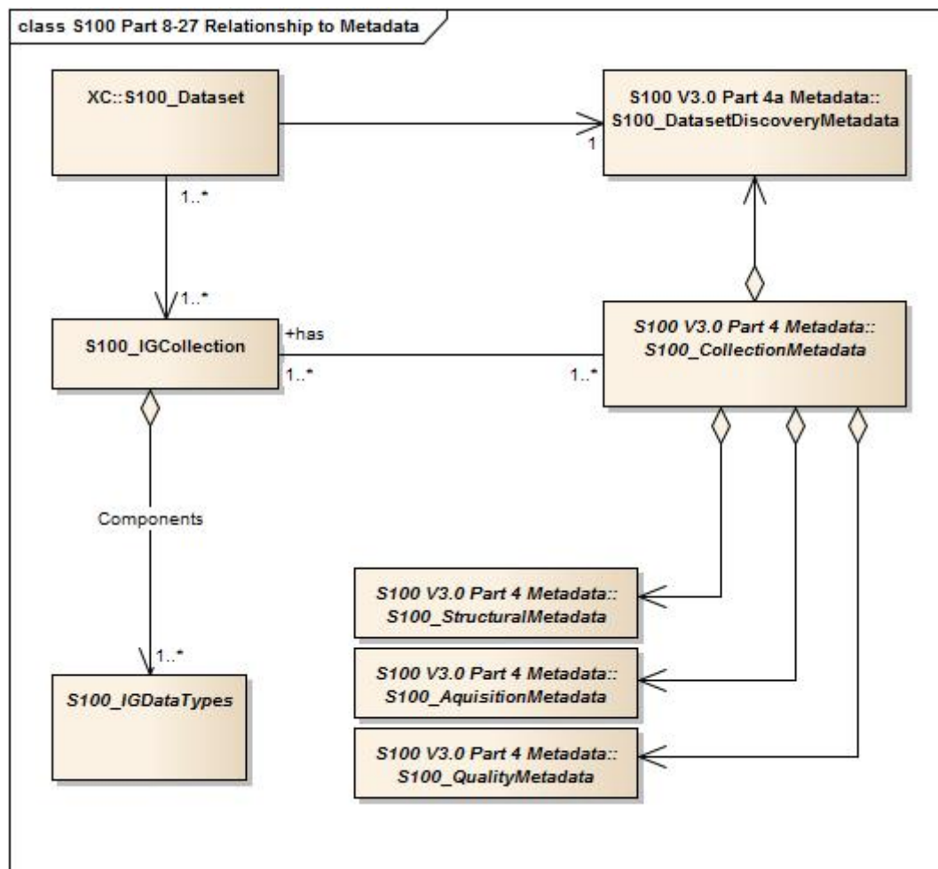
Figure 8-27 – Relationship to Metadata
