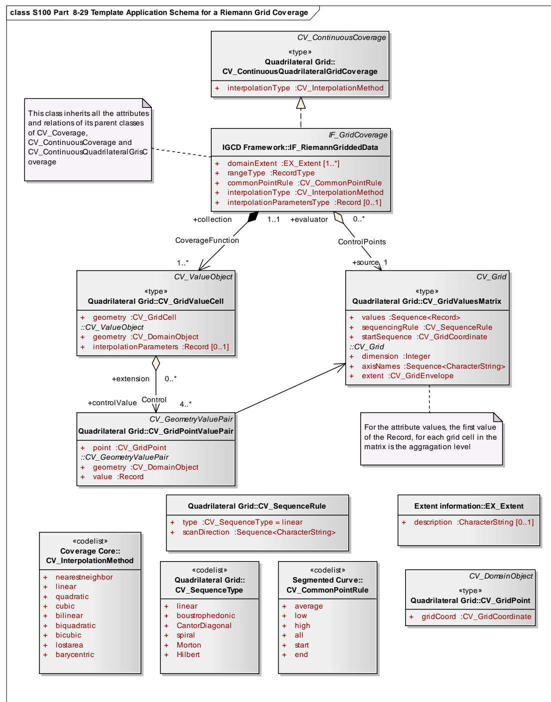
Figure 8-29 - Template Application Schema for a Riemann Grid Coverage
