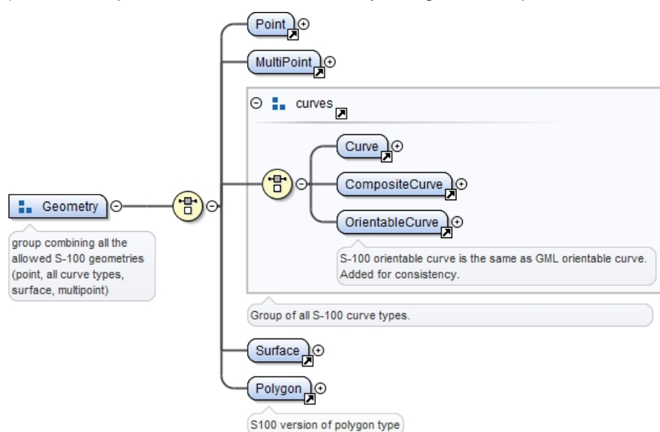
Figure 10b-8 – Geometry types defined in the base schema
