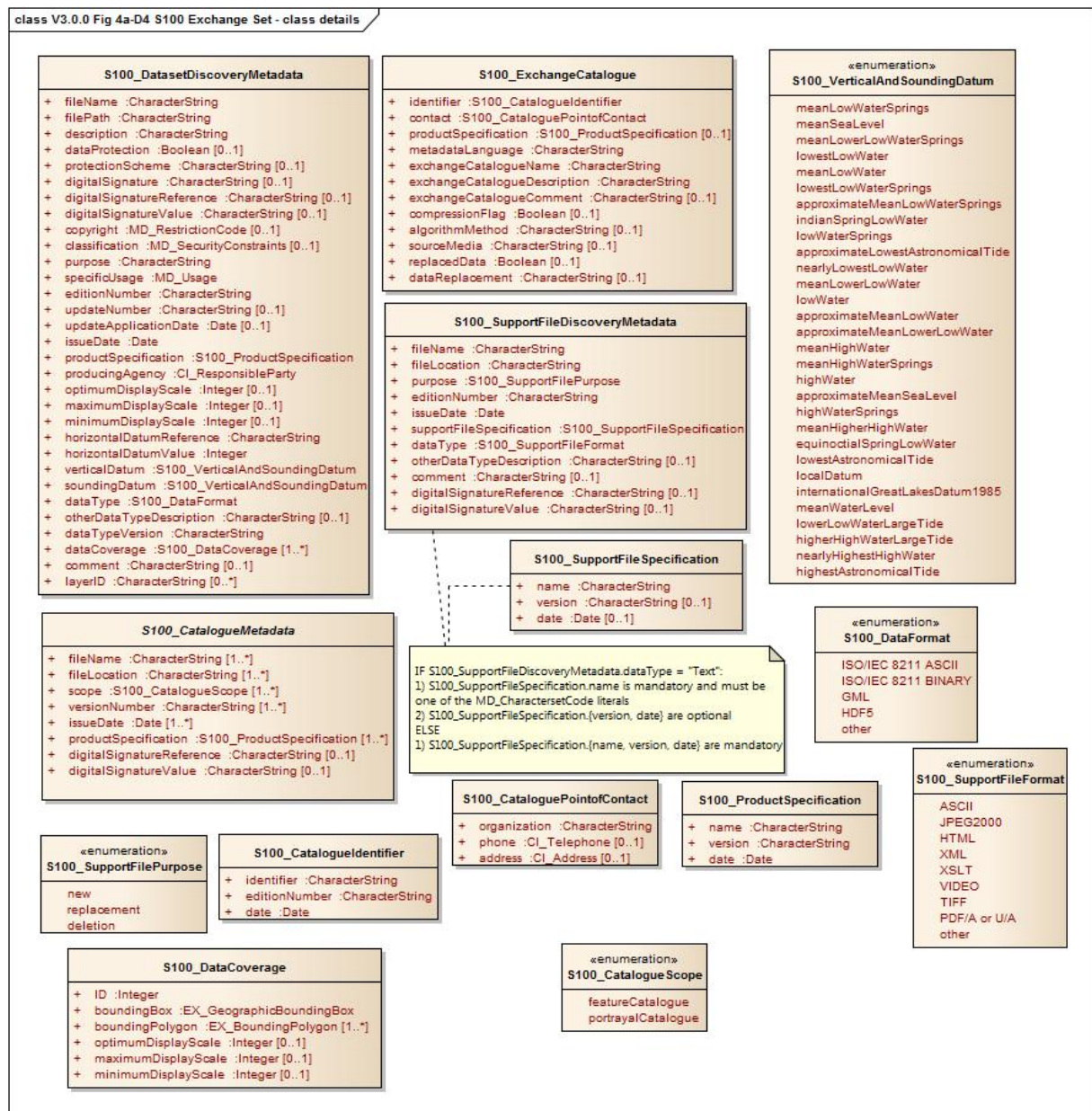
Figure 4a-D-4 S-100 Exchange Set - class details
