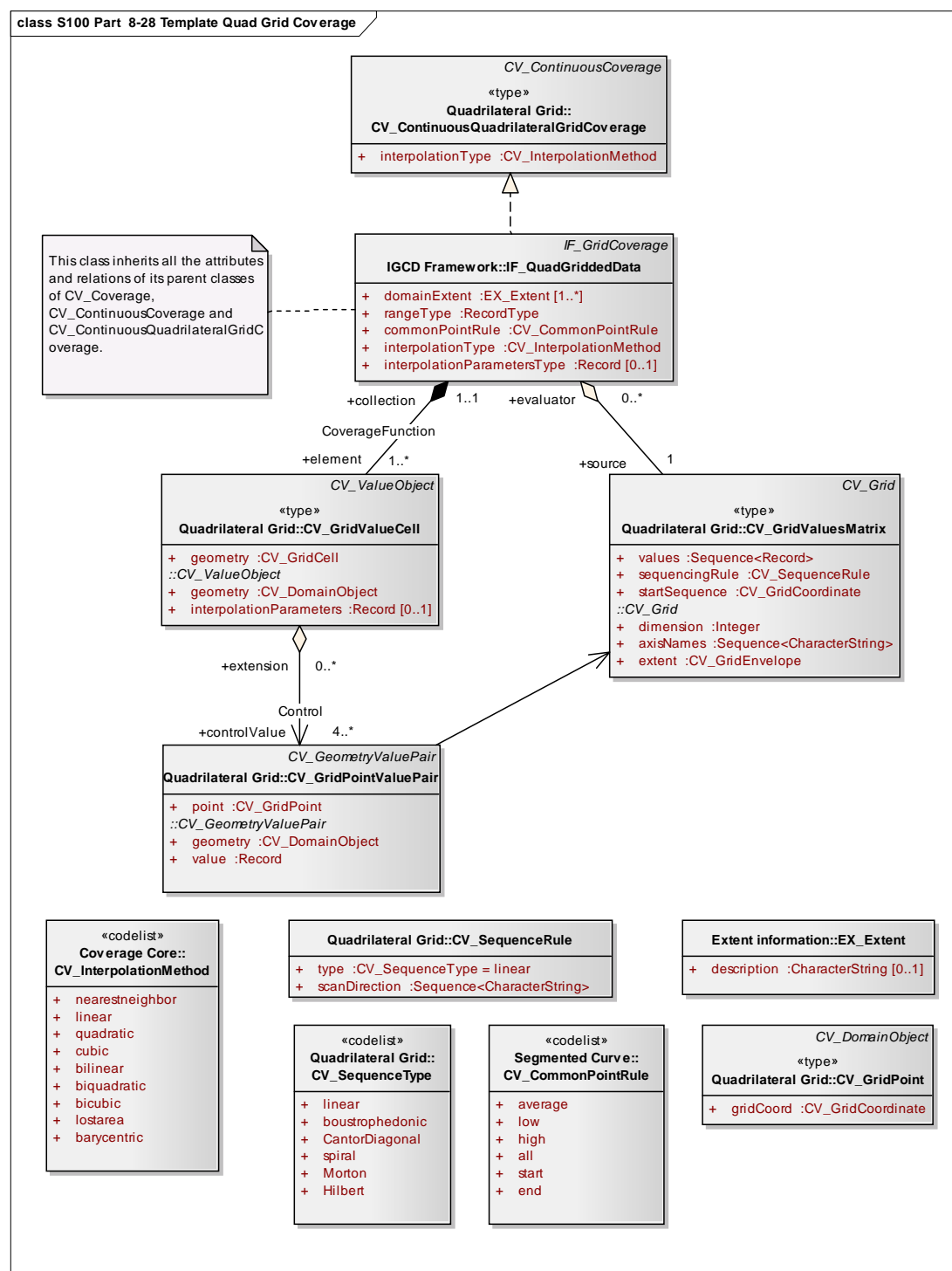
Figure 8-28 - Template Application Schema for a Quadrilateral Grid Coverage
