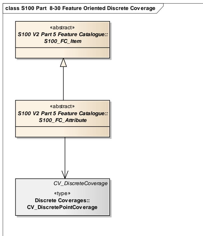
Figure 8-30 - Feature Oriented Discrete Coverage
