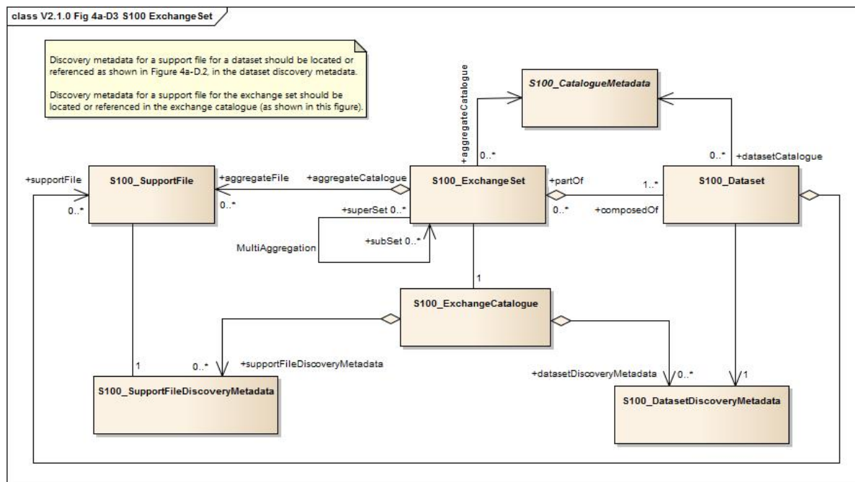
Figure 4a-D-3 – S-100 Exchange Set
