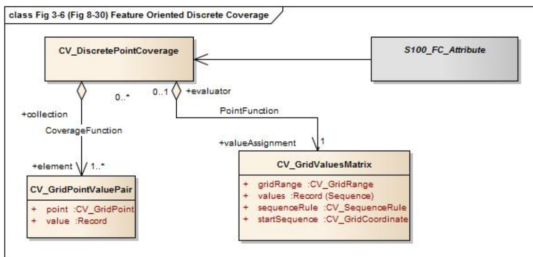
Figure 3-6 – Feature oriented discrete coverage
