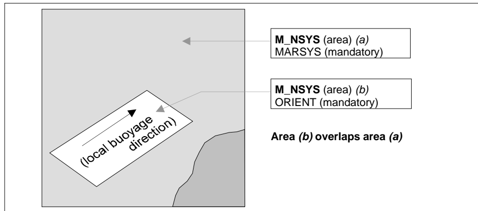
Figure 17 – Buoyage system and direction
