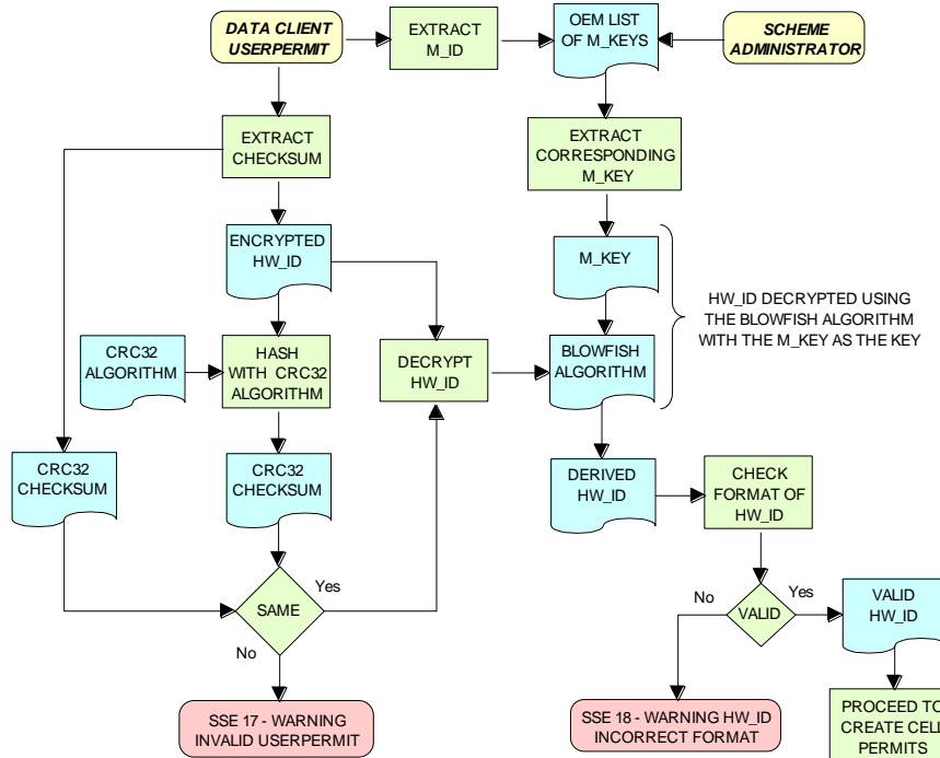
Data Server Process - Extract HW_ID from Userpermit
