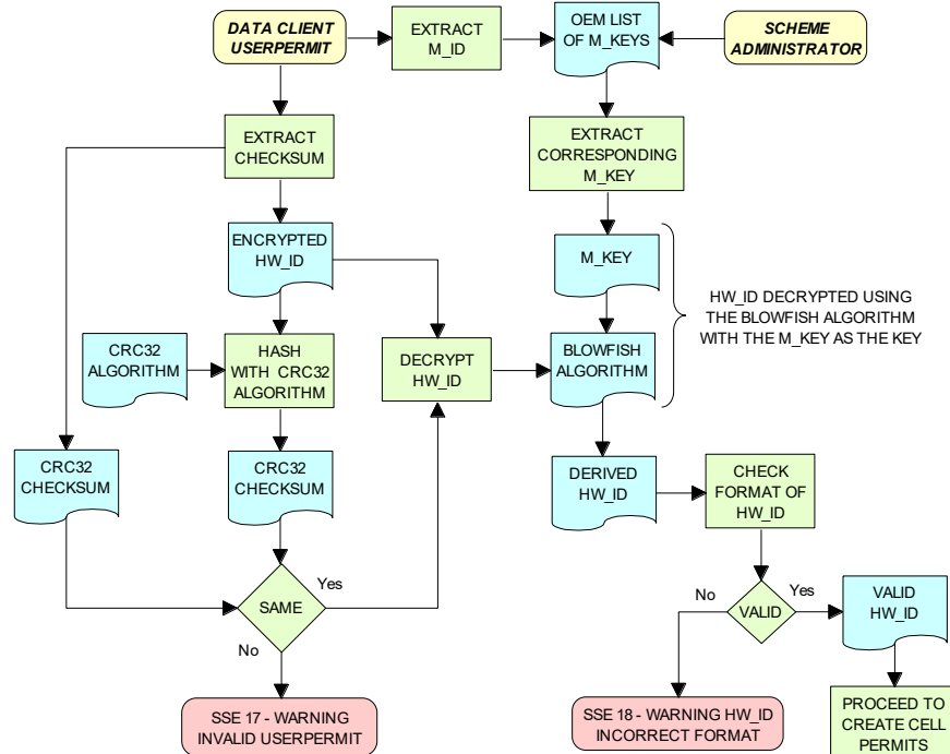
Data Server Process - Extract HW_ID from Userpermit
