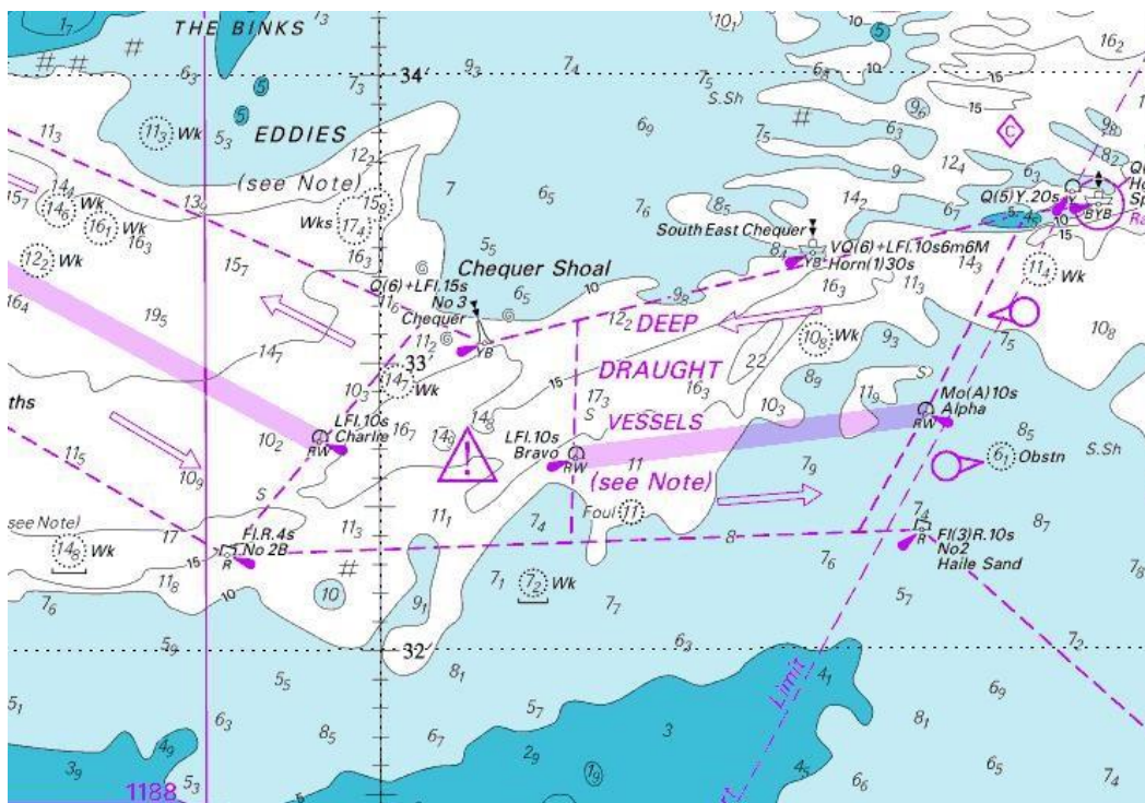
Figure 2-1 – Example of a raster chart
