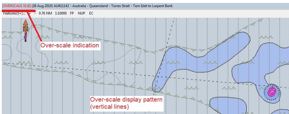
Figure 6-8 – Over-scale indication and over-scale pattern on ECDIS Source: AHO.
