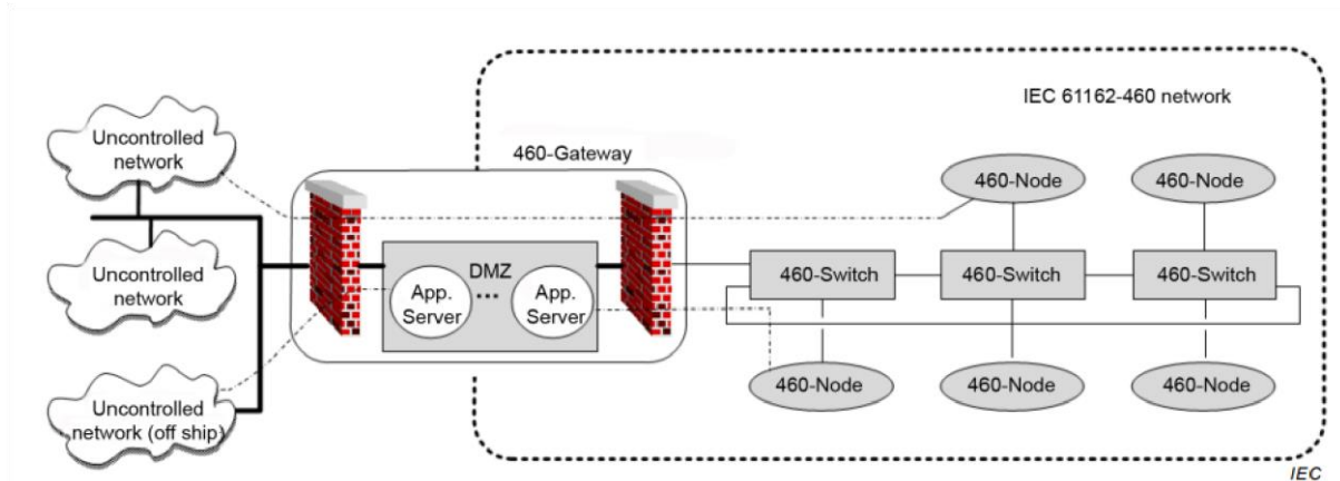
Figure 10-2 – Establishment of security zones
