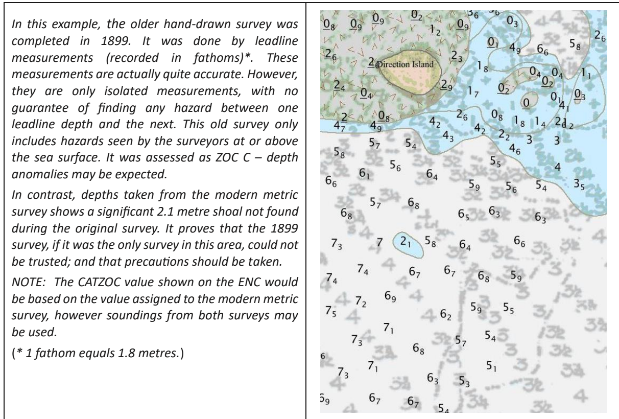
Figure B-2 – Example: Leadline survey from 1899
