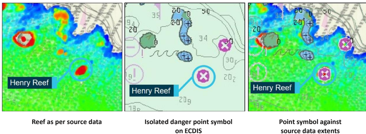
Figure 6-5 – Comparison of small reef within source data at ENC compilation scale, point symbol depiction on ENC, and source data overlaid on ENC Images show survey data (left), section of ENC (centre) and ENC superimposed on survey data at compilation scale (right). Source: Australian Hydrographic Office (AHO) and ATSB 3 .
